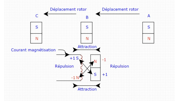
Fig. 2. Sequence of rotor displacement (positions A, B, C) facing the electromagnet with a neodymium core whose own field is cancelled by superposition. The diagram uses the same polarity and crossed-interaction convention as Figure 1.
